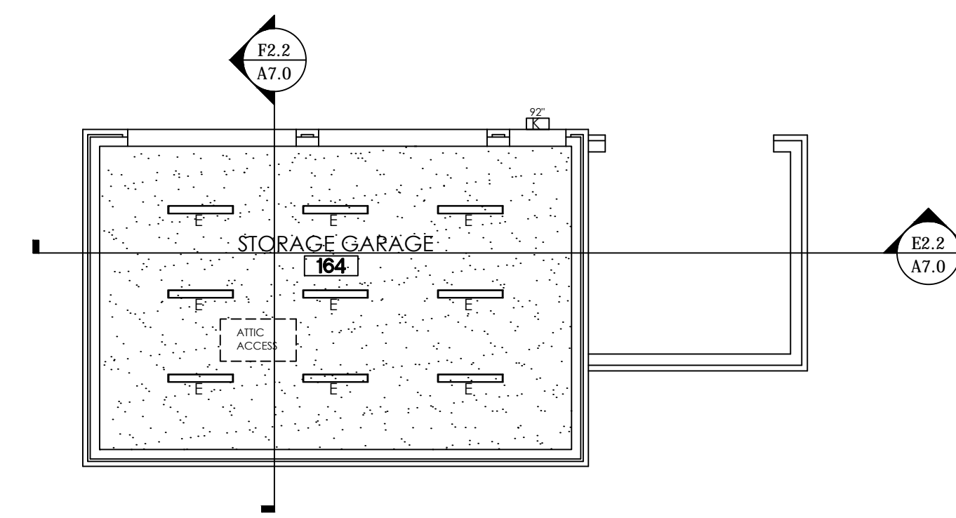
REFLECTED CEILING PLAN - STORAGE GARAGE SCALE: 1/8" = 1'-0"
